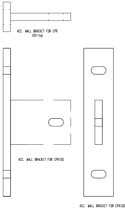
WALL BRACKET FOR 100-V VERTICAL
