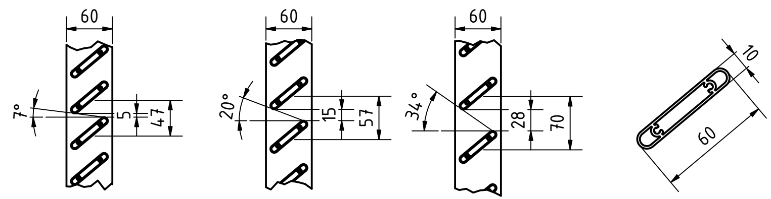
M ( 1 : 5 ) Standard center to center
