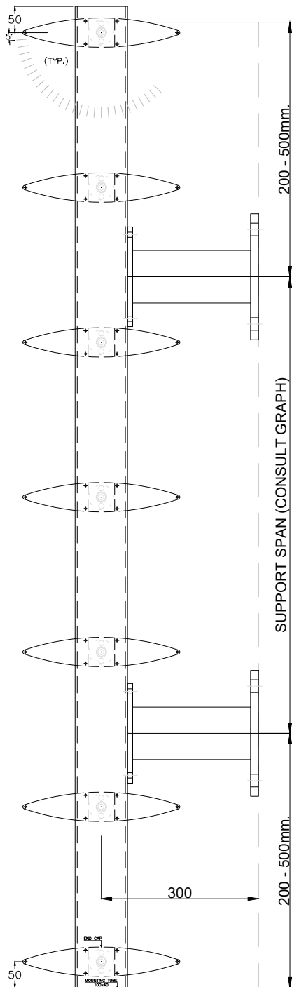
FIXED SYSTEM ON TUBE
